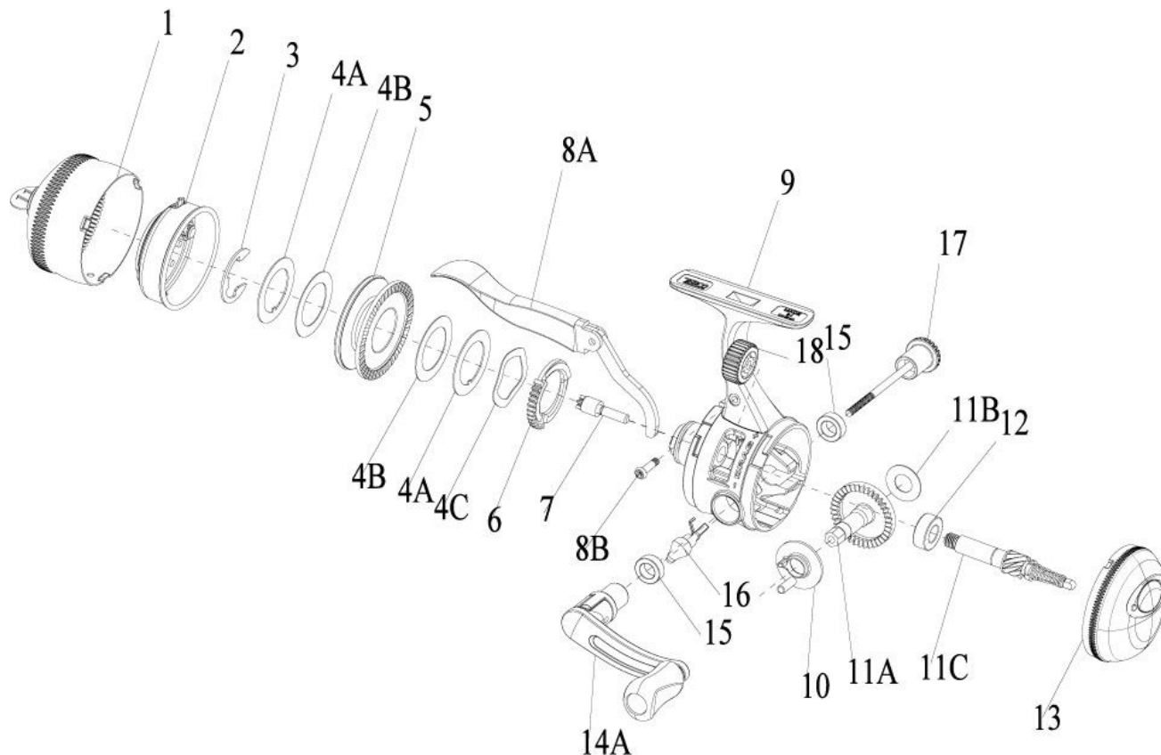
Zebco 11 Micro Triggerspin Authentic Spincast Reel Part List
